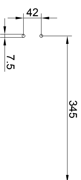
Drilling Scheme
