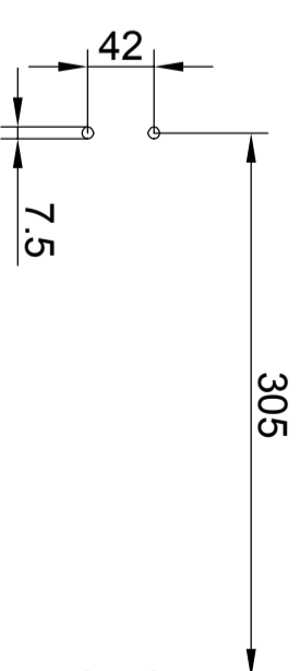
Drilling Scheme
