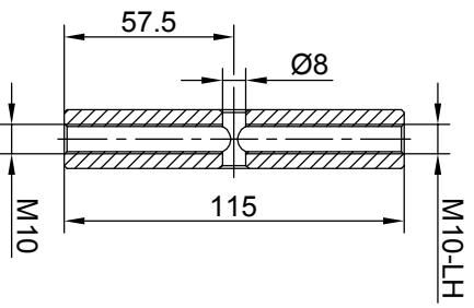
Coupling screw
