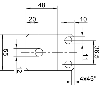
Deck fixture
